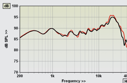
ABOVE: The forward response's 'brightened' presence and treble can be tamed by toeing-in the speakers
