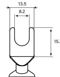
U-Spade Dimensions (mm)
