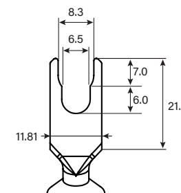
Multi-Spade Dimensions (mm)
