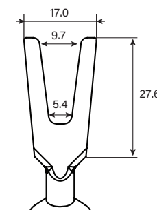
V-Spade Dimensions (mm)
