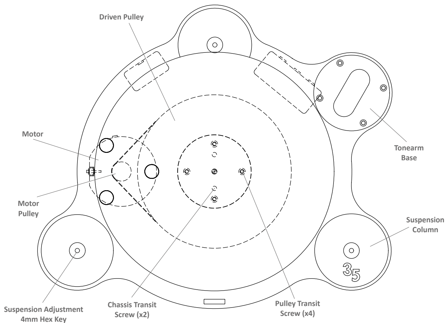
PLAN VIEW Figure 1
