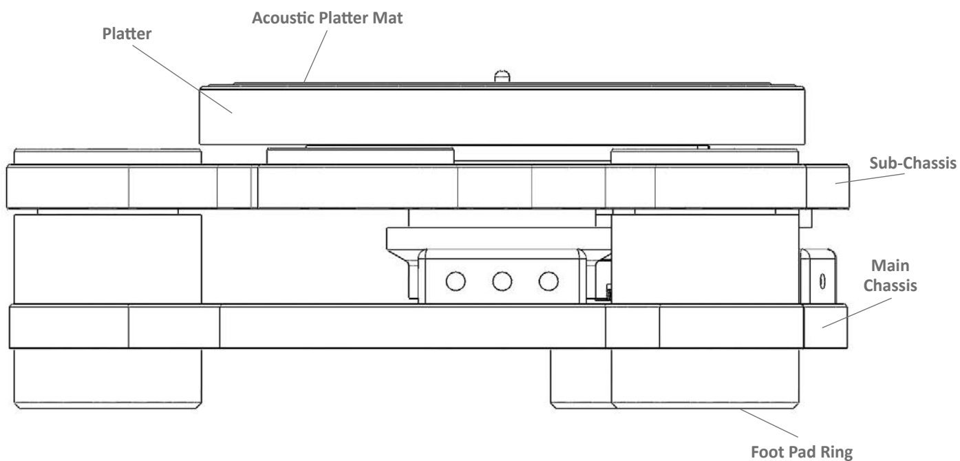
SIDE VIEW L/H Figure 4
