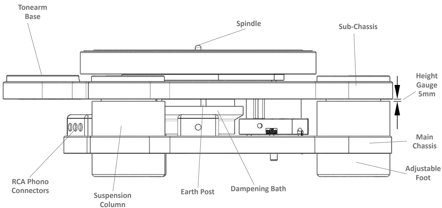
SIDE VIEW R/H Figure 3
